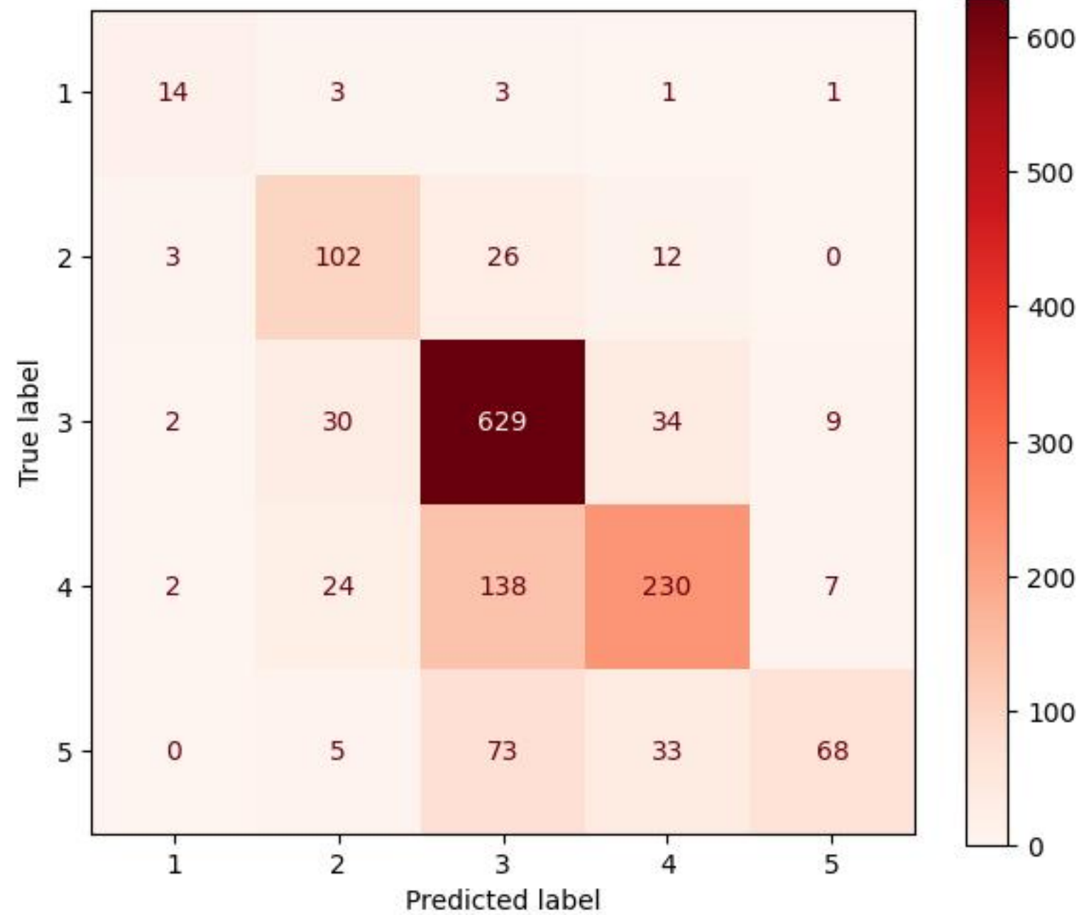
Overfit Model: Train Confusion Matrix
