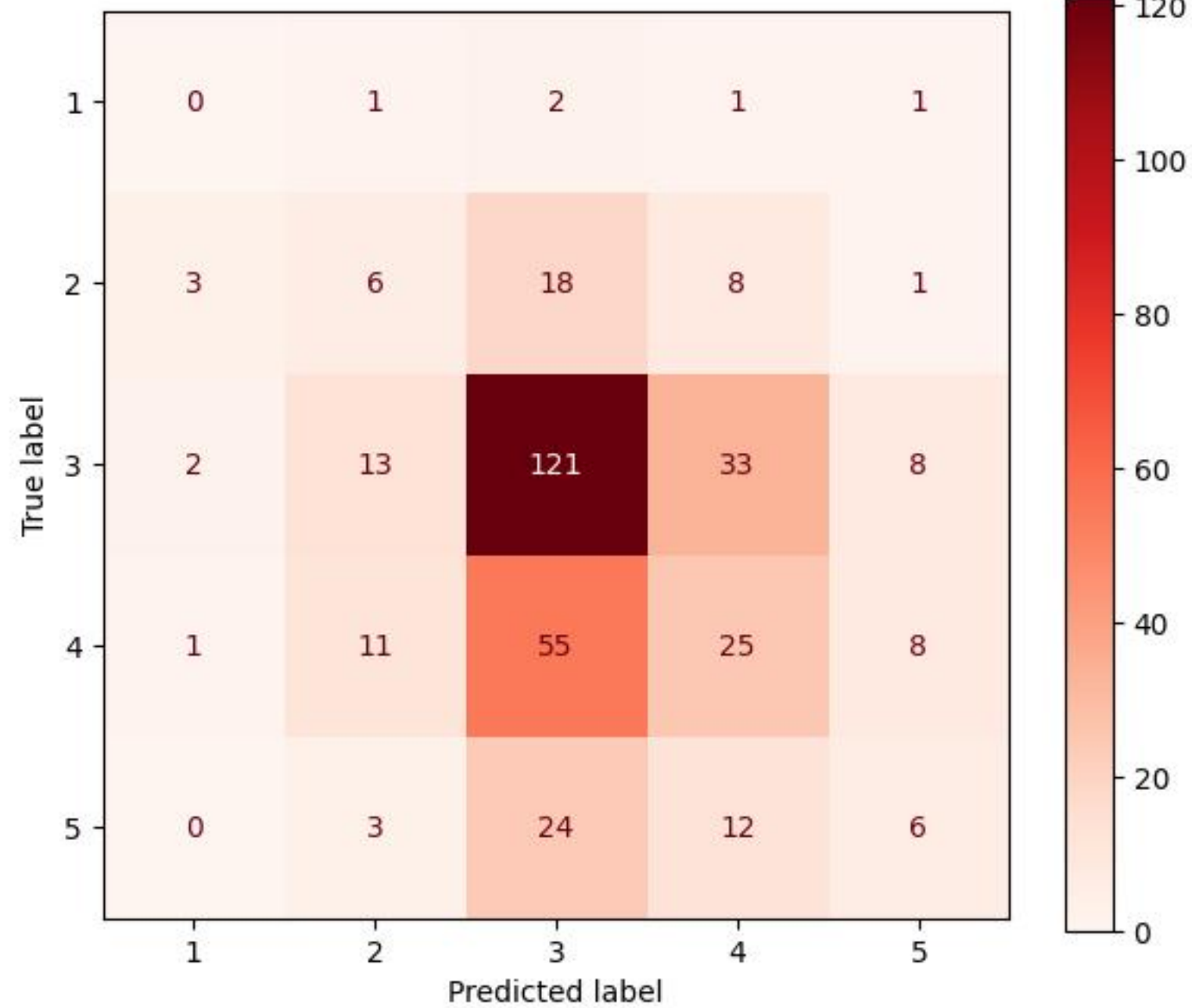
Overfit Model: Test Confusion Matrix
